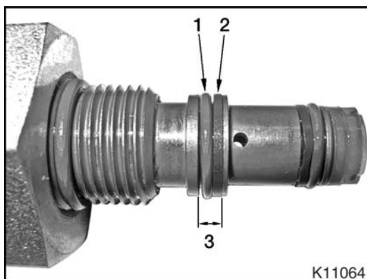
Figure 1 IPR valve (old)
